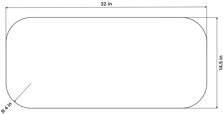
OBJECT 005 - SIDE
